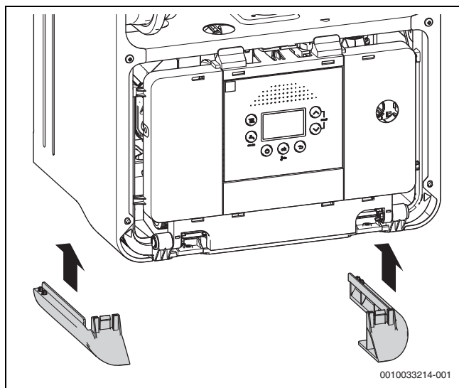
Fig. 68 Colocar as barras de plástico laterais
