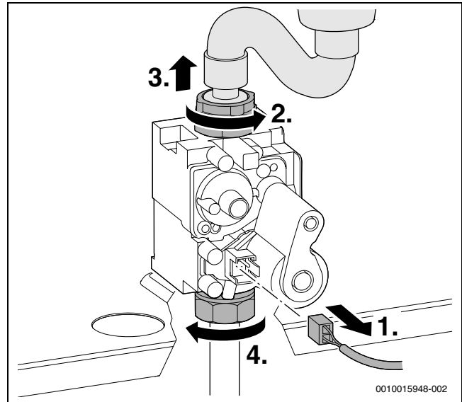
Fig. 58 Retirar as fichas e soltar as porcas de capa
